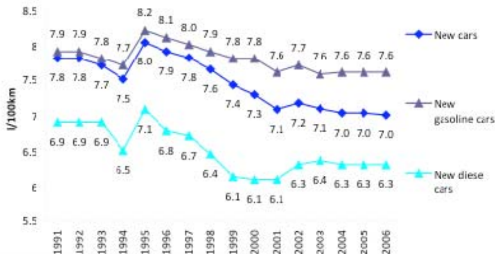
Figure 13: Specific fuel consumption of cars (new vehicles)
