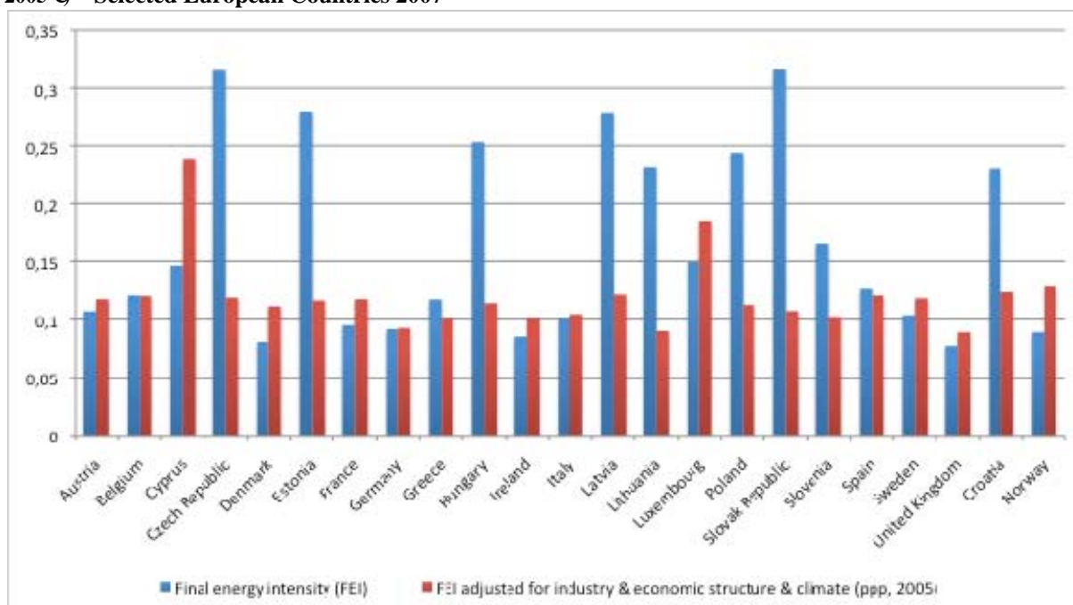
Figure 10: Final energy intensity (FEI) vs. FEI adjusted for economic structure, climate & PPP (koe per one 2005 €) – Selected European Countries 2007
