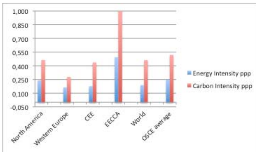
Figure 19: Energy and carbon intensities (2008) (left axis: koe or kCO 2 per 2005 U.S. Dollar)
