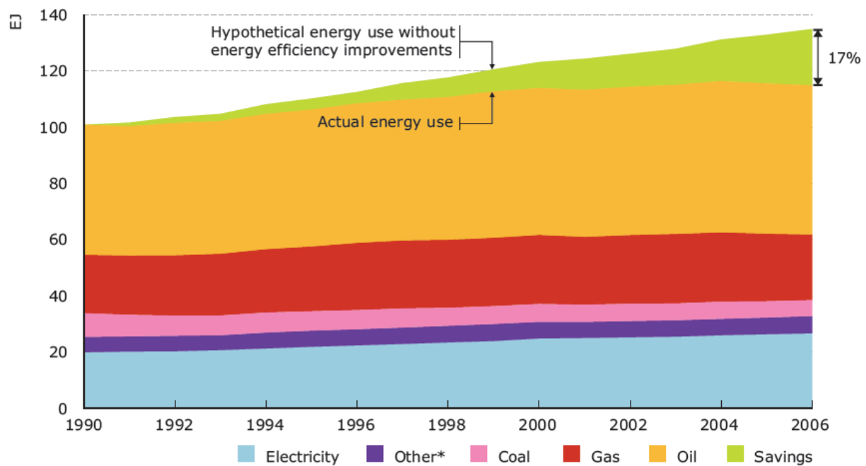
Figure 23: Energy savings from improvements in energy efficiency, IEA17
