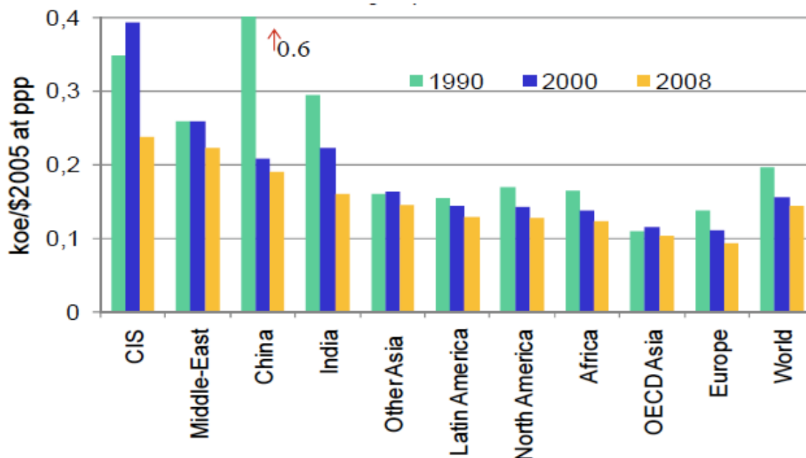
Figure 11: Energy intensity of industry in 1990, 2000 and 2008 in selected countries and regions (PPP)
